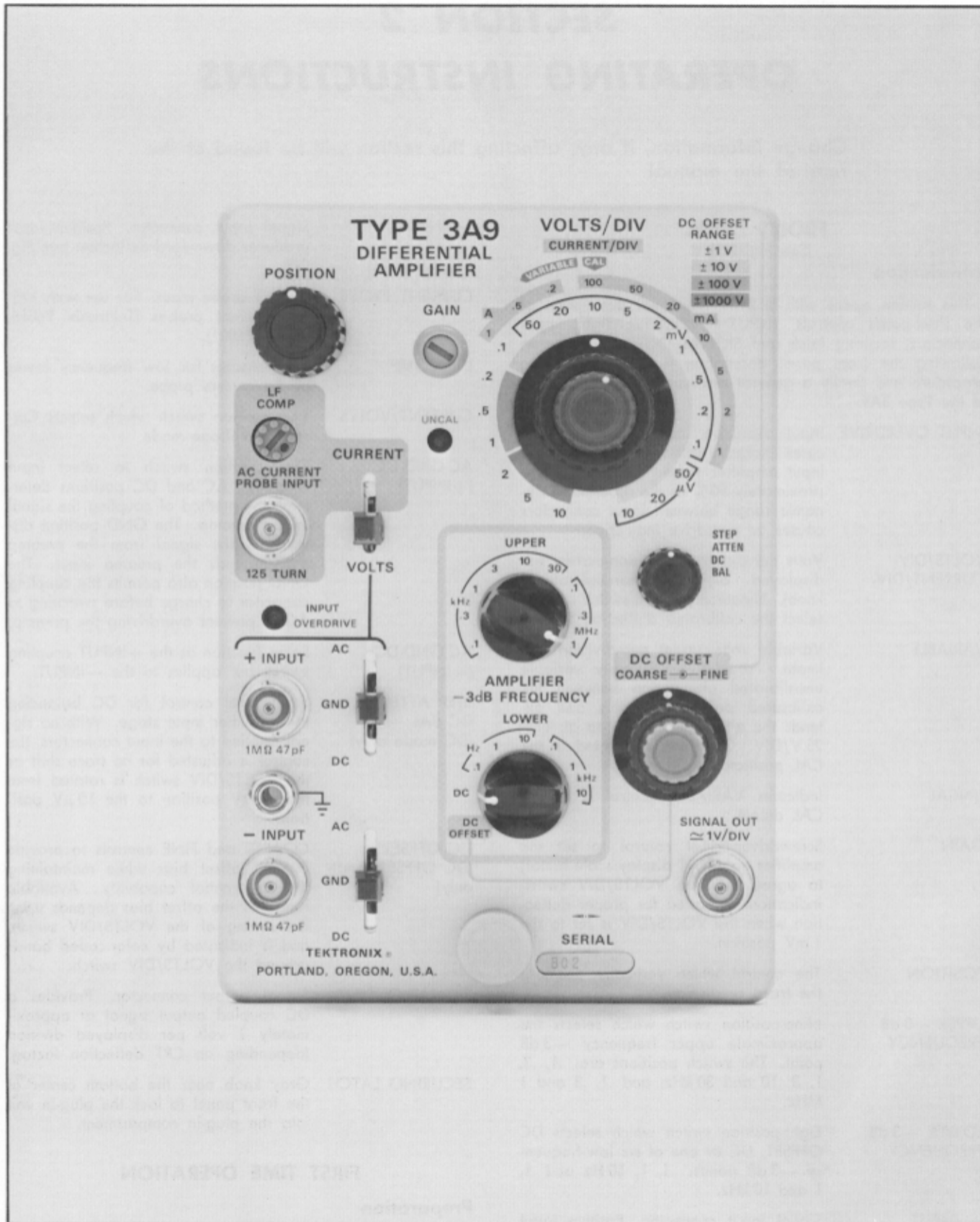
Fig. 2-1. Front-panel controls.
